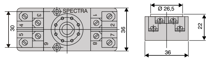
8 Pin
