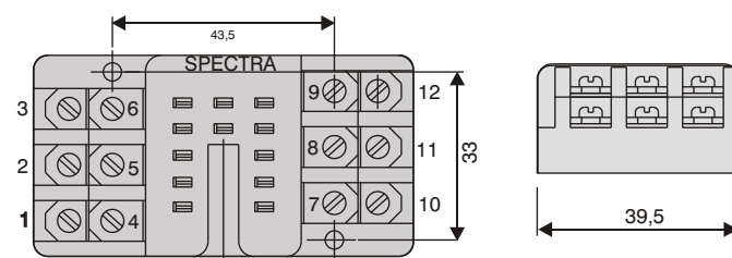
11 Pin -3R4R
