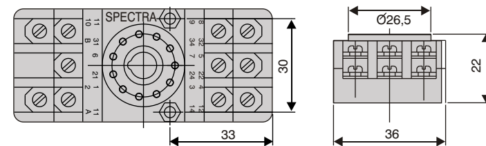
11 Pin
